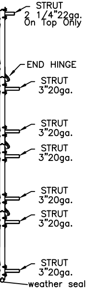
SECTION "B-B"
