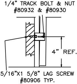
DETAIL D
